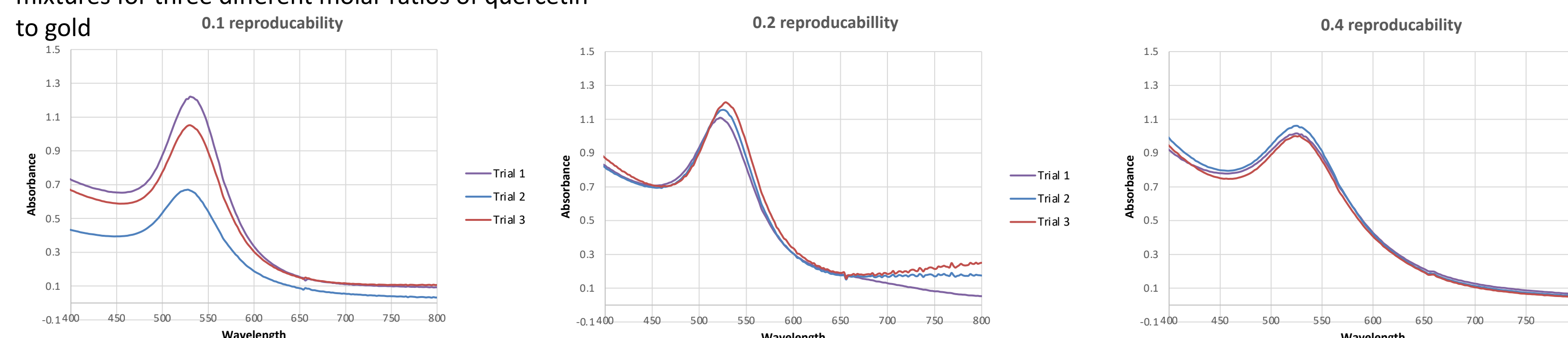
Figure 5 (left) UV-vis spectra from three replicates with 0.1:1 molar ratio; (middle) UV-vis spectra from three replicates with 0.2:1 molar ratio; (right) UV-vis spectra from three replicates with 0.4:1 molar ratio
