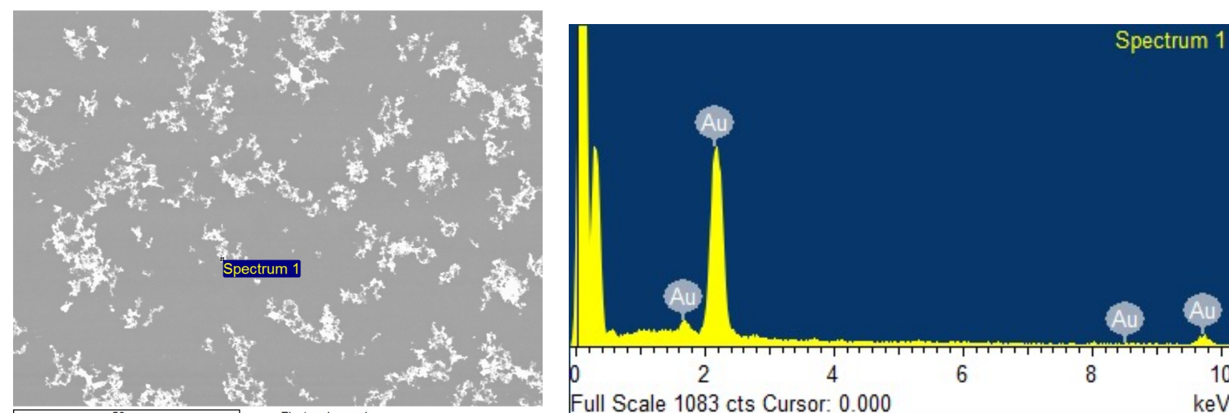
Figure 2. (left) SEM image and (right) EDX analysis of redispersed gold nanoparticles prepared with a 0.2:1 molar ratio of quercetin to gold.
